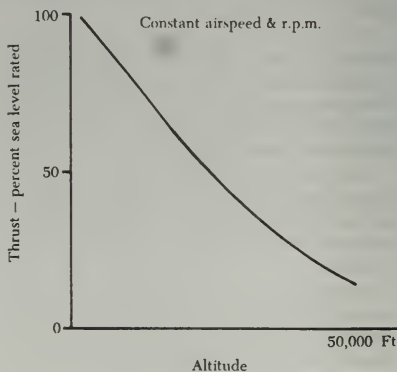
FIGURE 1-75. Effect of altitude on thrust output.
